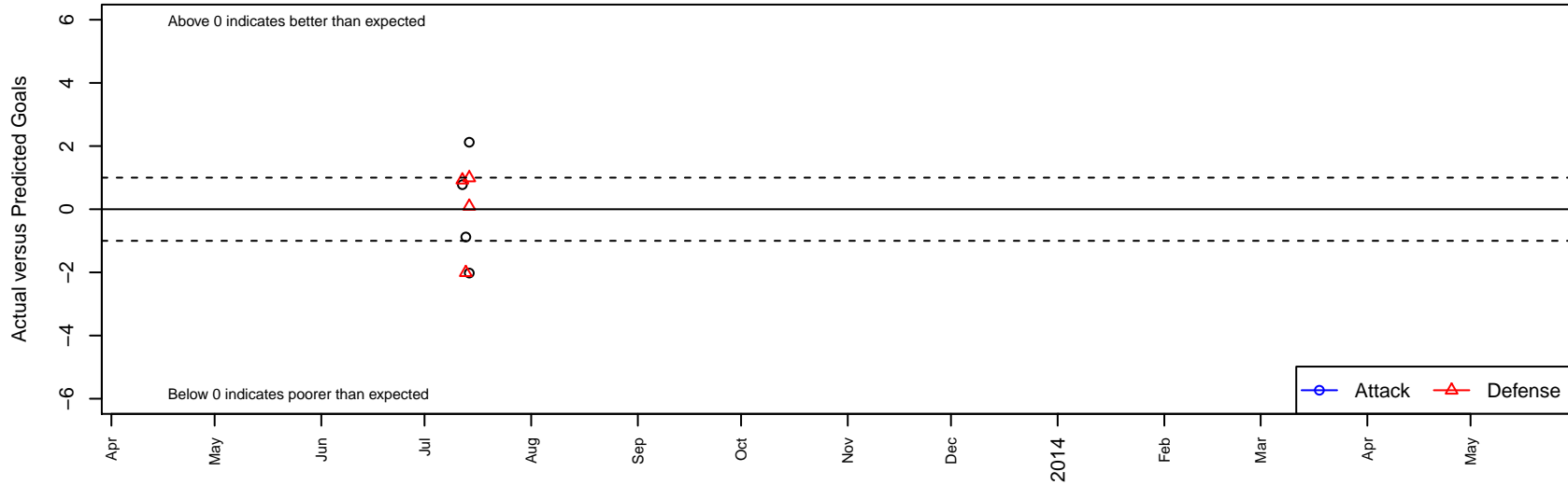
Crossfire Oregon –Unk B98 Dots are actual minus expected GF (blue circles) and GA (red triangles). Blue line is smoothed change in attack strength. Red is smoothed change in defense strength.
